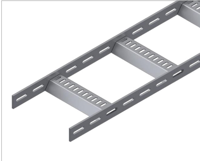
12 VD Cable Ladder with 40x5mm Roll Profile Lama / Down Type
