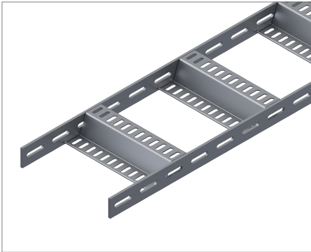
12 Z70 Cable Ladder with 40x5mm Roll Profile Lama
