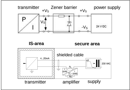
Fig. 2 circuit diagrams
