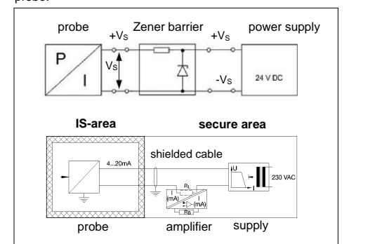
Fig. 4 circuit diagrams
